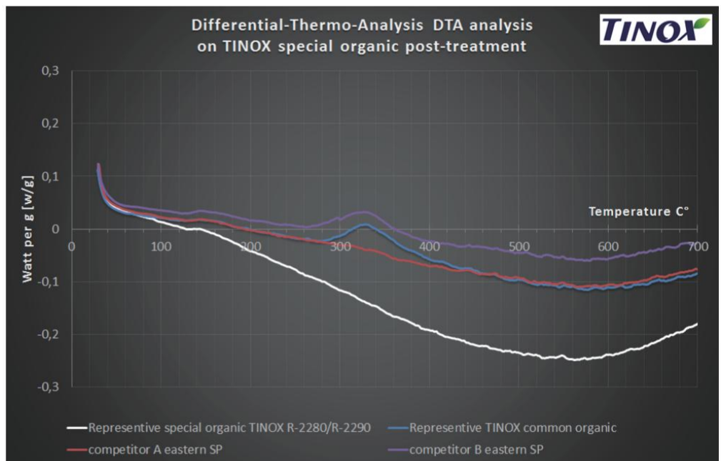
Fig.3: Differential-Thermo-Analysis DTA analysis on TINOX special organic post-treatment
